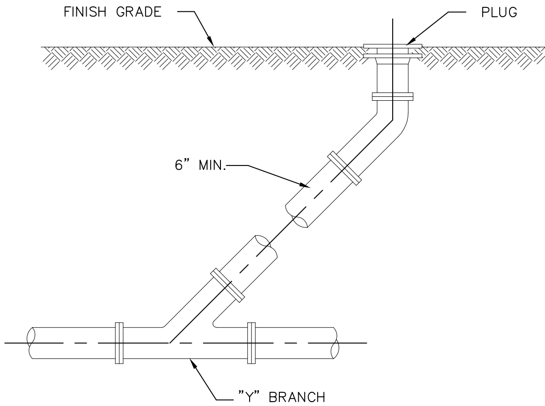
SANITARY SEWER CLEANOUT
